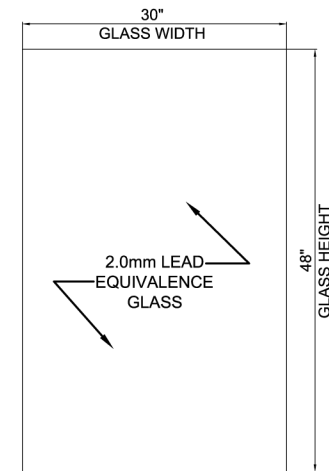
B 1 GLASS ELEVATION
