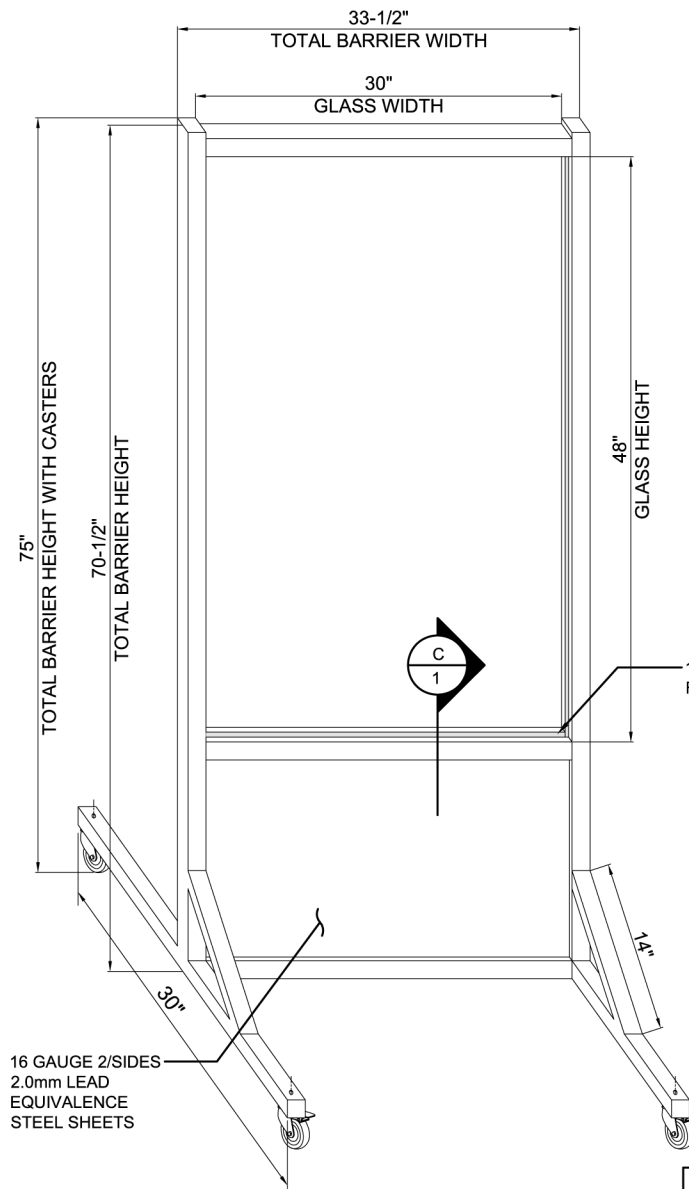
A 1 BARRIER ELEVATION
